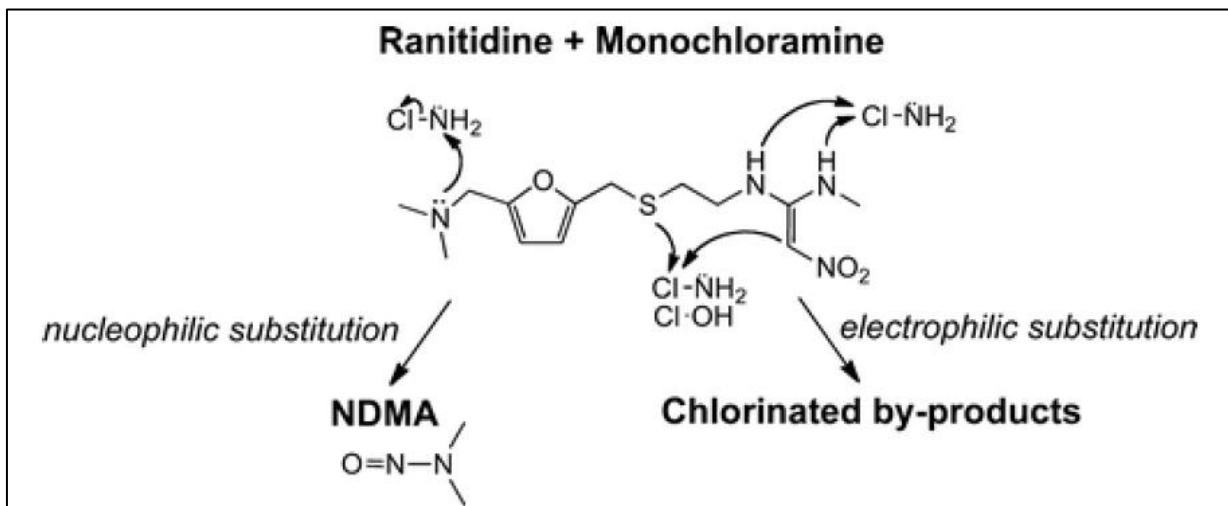
16 Figure 3 –Mechanism for Decomposition of Ranitidine in NDMA
