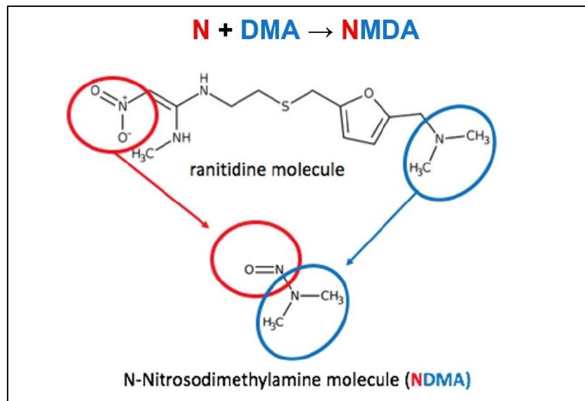
10 Figure 1 –Ranitidine Structure & Formation of NDMA
