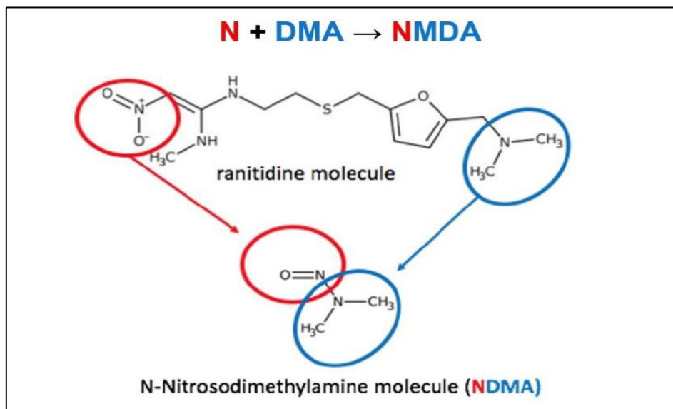
Figure 1 –Ranitidine Structure &amp; Formation of NDMA
