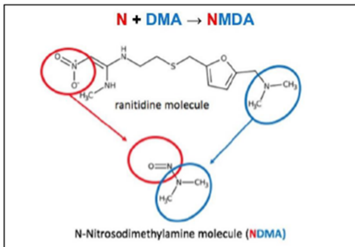
Figure 1 –Ranitidine Structure & Formation of NDMA
