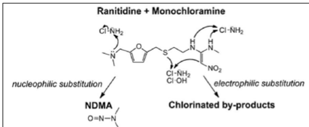
Figure 2 –Mechanism for Decomposition of Ranitidine in NDMA
